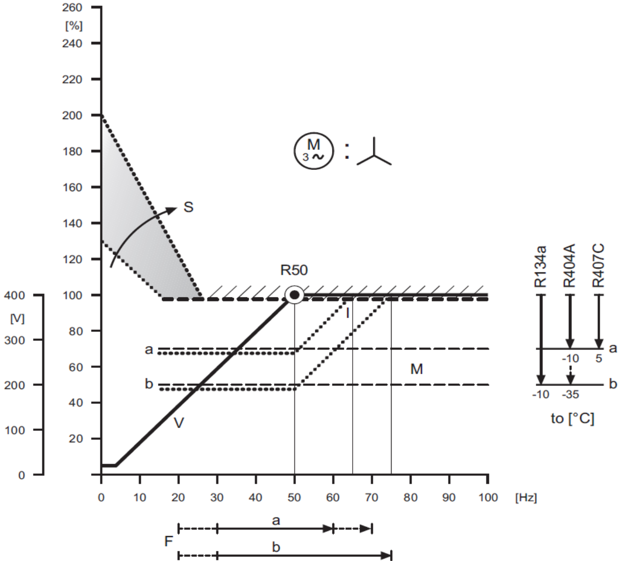
Fig 4.1a: Standard motor connection; Operation with 400 V / 50 Hz supply (Example)
