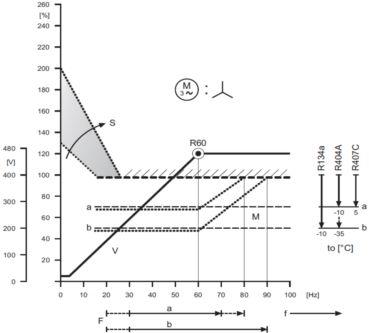
Fig 4.1b: Standard motor connection; Operation with 460 V / 60 Hz supply
