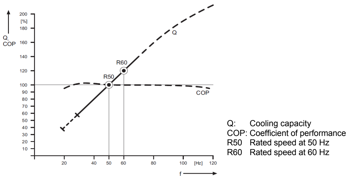
Fig 3.2: Cooling performance of a typical positive-displacement, reciprocating, refrigerant compressor over the permissible frequency range at steady-state operation
