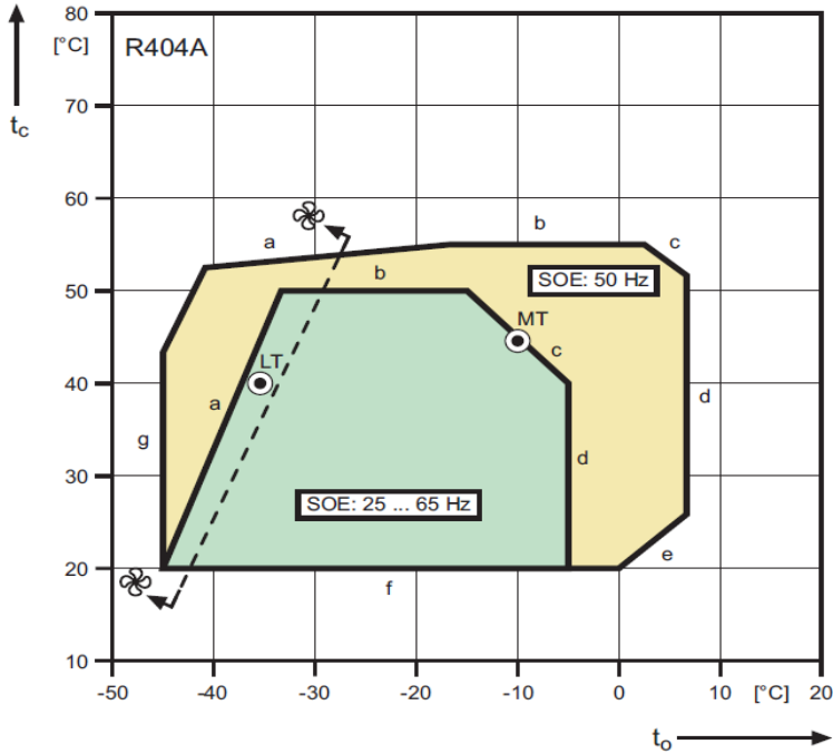
Fig 4.2a: R404A; Large motor; Standard connection; 400 V / 50 Hz supply (Example)
