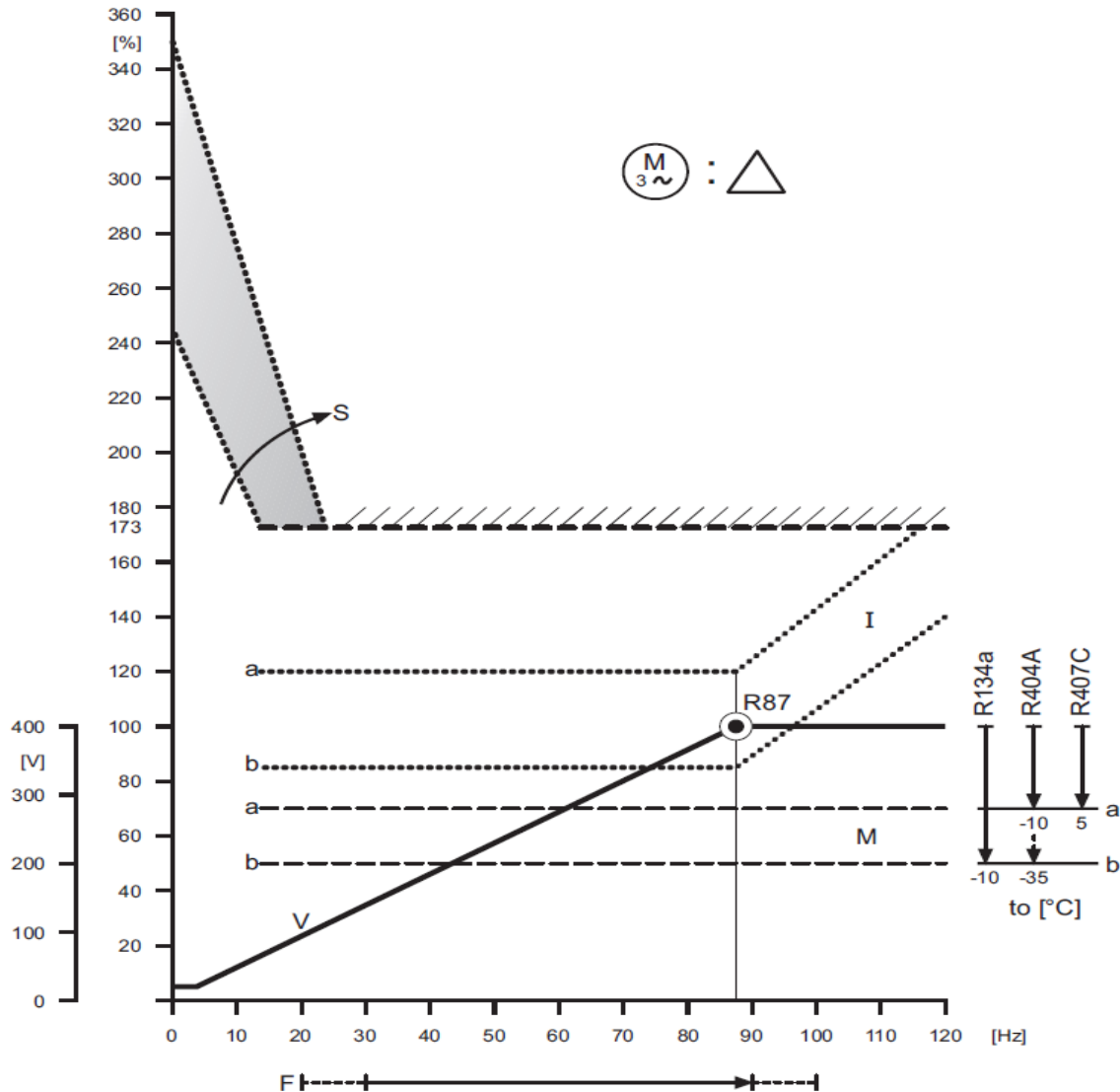
Fig 4.1c: Special 87 Hz motor connection; Operation with 400 V / 50 Hz supply
