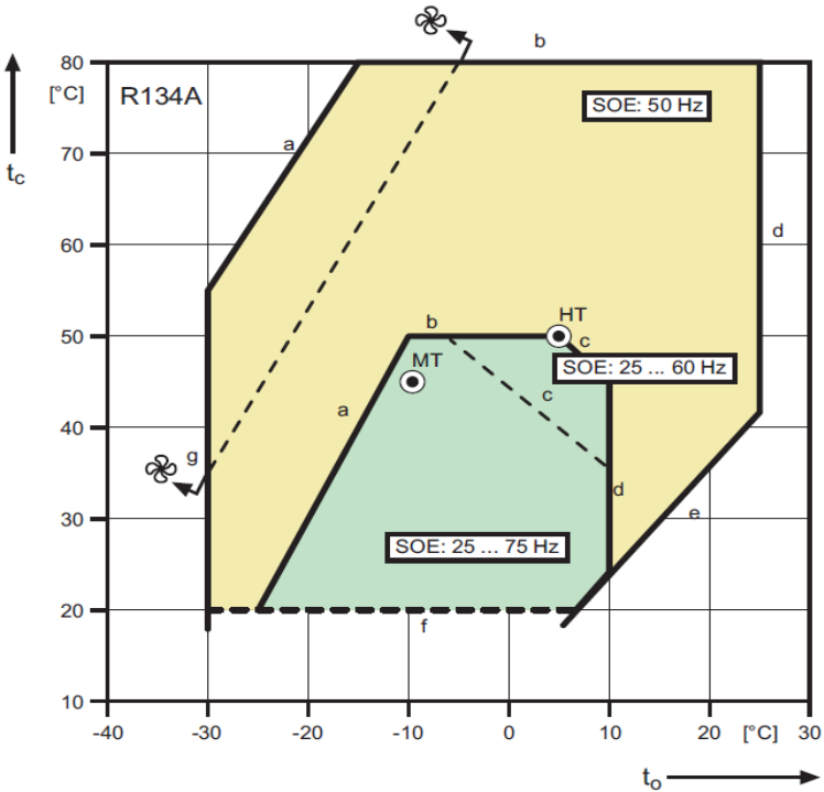
Fig 4.2b: R134a; Standard connection; Operation with 400 V / 50 Hz supply (Example)
