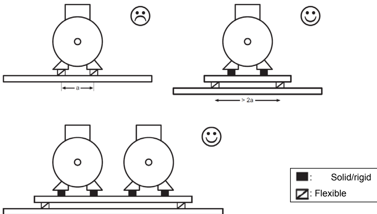
Fig 5.3: Mounting of reciprocating compressors for variable-speed operation (Example with 2-cylinder reciprocating compressors)
