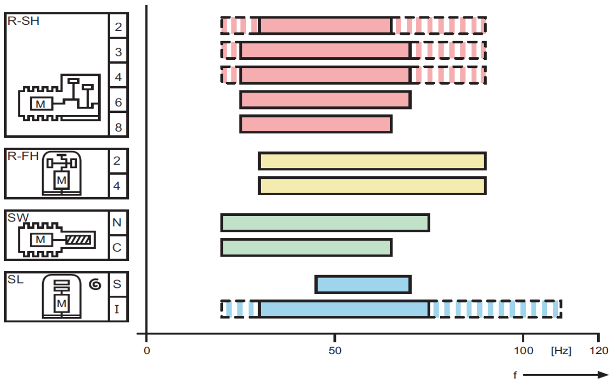
Fig 5.1: Typical permissible ranges of frequency for different types of compressor
