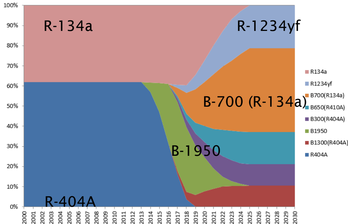
GasInNewUnits, tonnes, Low Estimate, Commercial Refrig, Single condensing units MT
